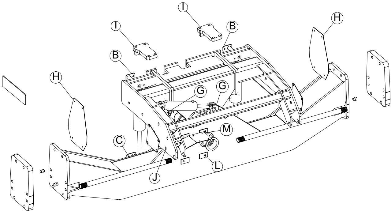
REAR VIEW
