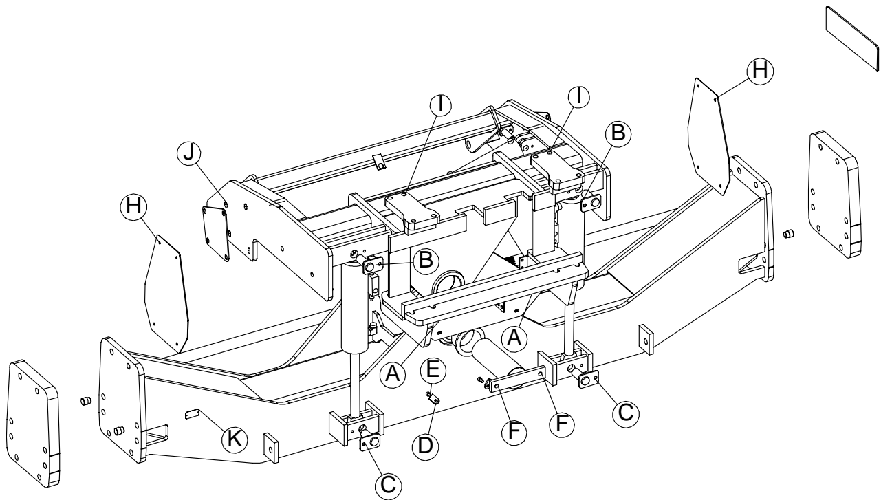
REAR VIEW
