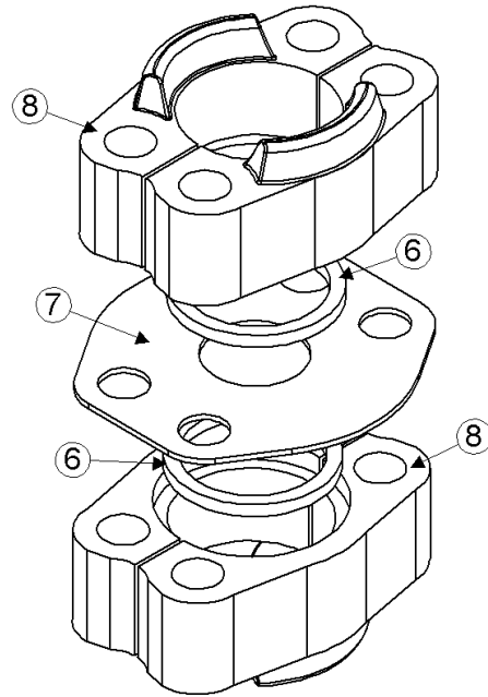
CODE 62 SPLIT FLANGE CONNECTOR KIT ASSEMBLY WITH O-RINGS
