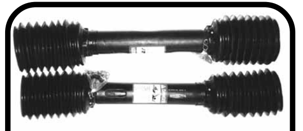
Hillco Conversion Kits use high quality Walterscheid 2400 series drivelines
